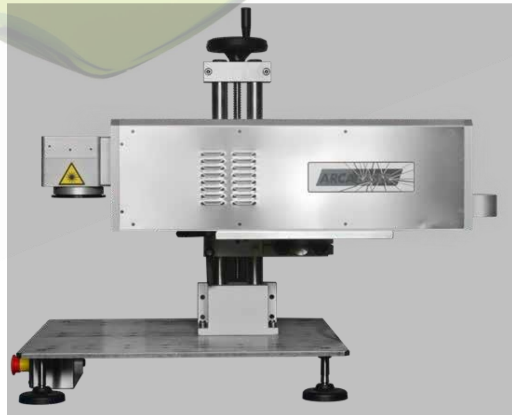
Complete with a vertical recirculating ball screw adjustment and horizontal adjustment (both with millimetric references). The base is perforated for the easy positioning of possible templates
